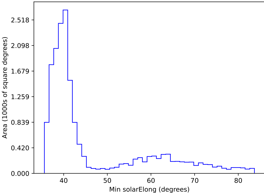
too_ignore_10_1v3.4_10yrs WFD all bands: Min solarElong
