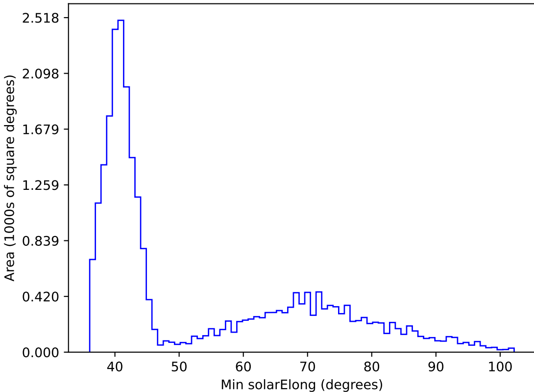
too_ignore_10_1v3.4_10yrs All sky z band: Min solarElong
