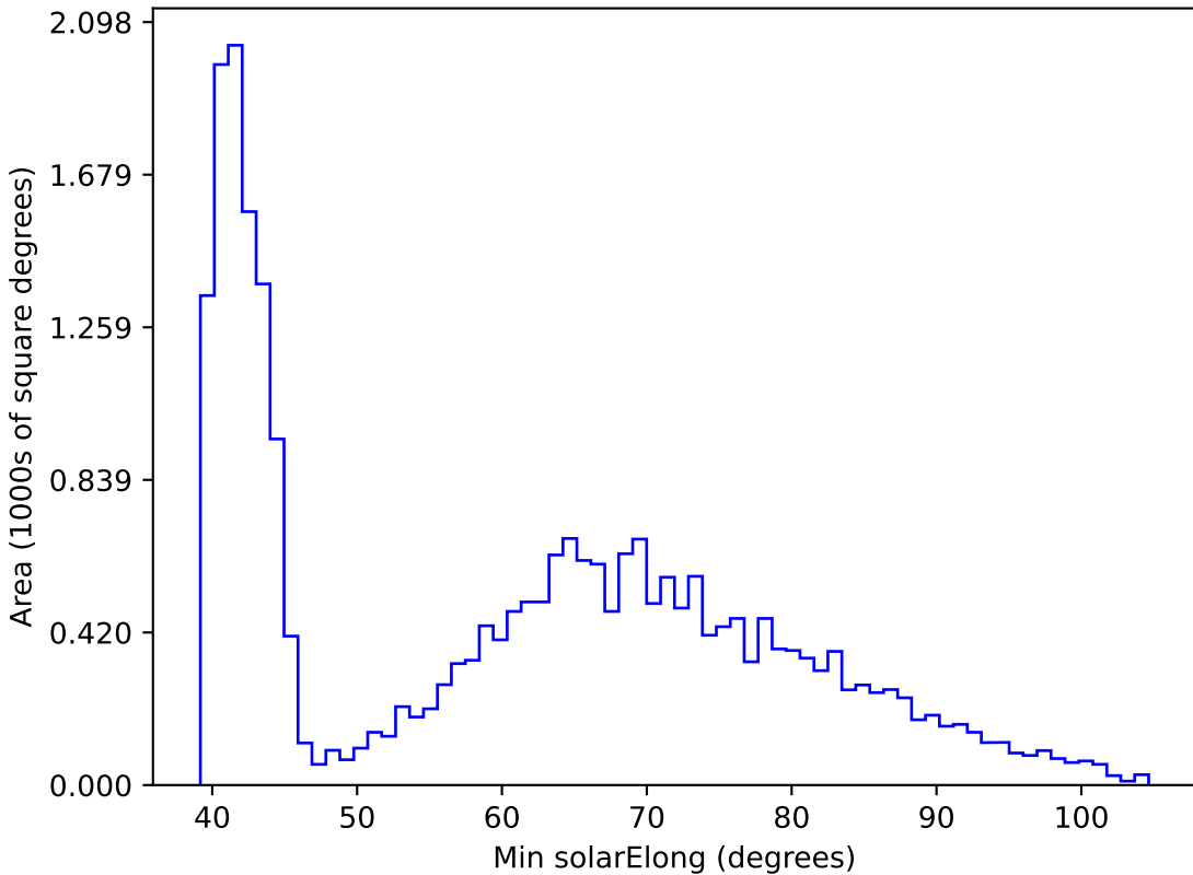
too_ignore_10_1v3.4_10yrs All sky r band: Min solarElong
