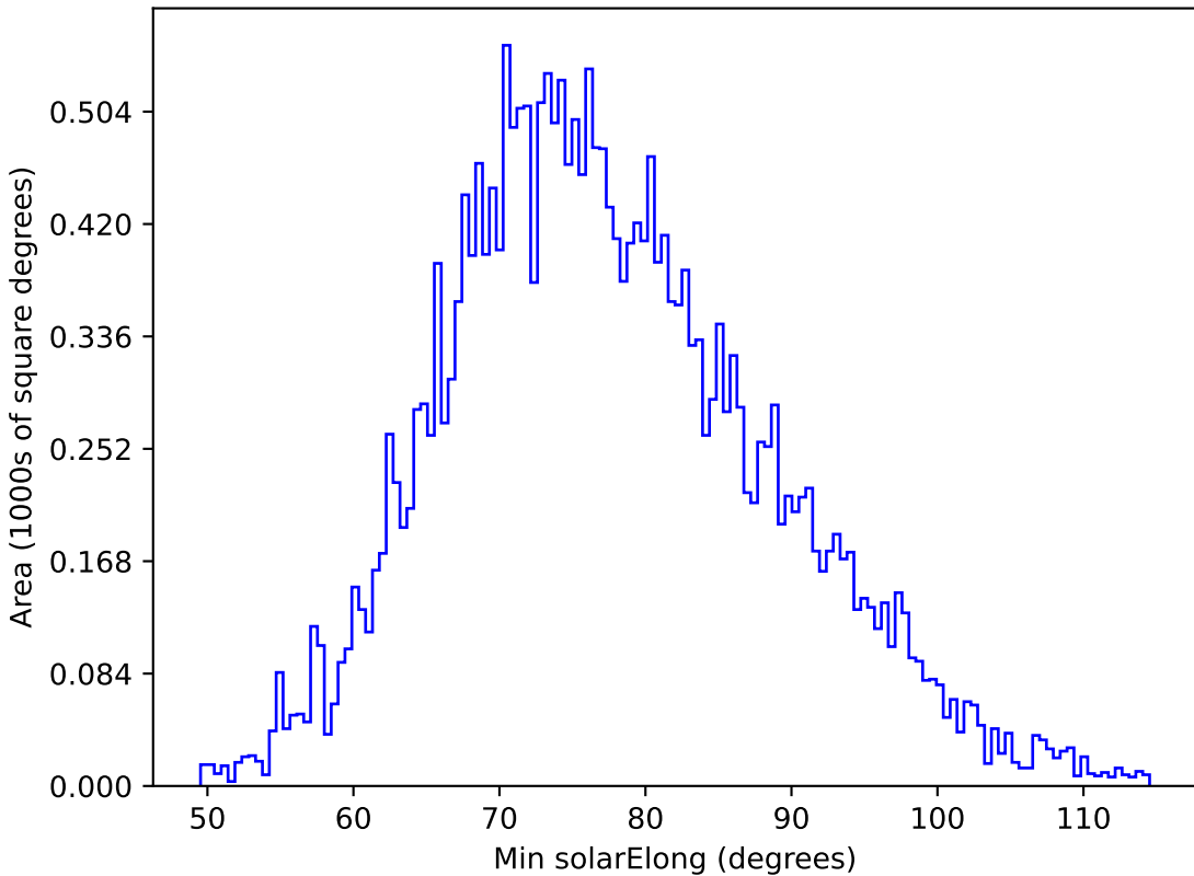
too_ignore_10_1v3.4_10yrs All sky g band: Min solarElong
