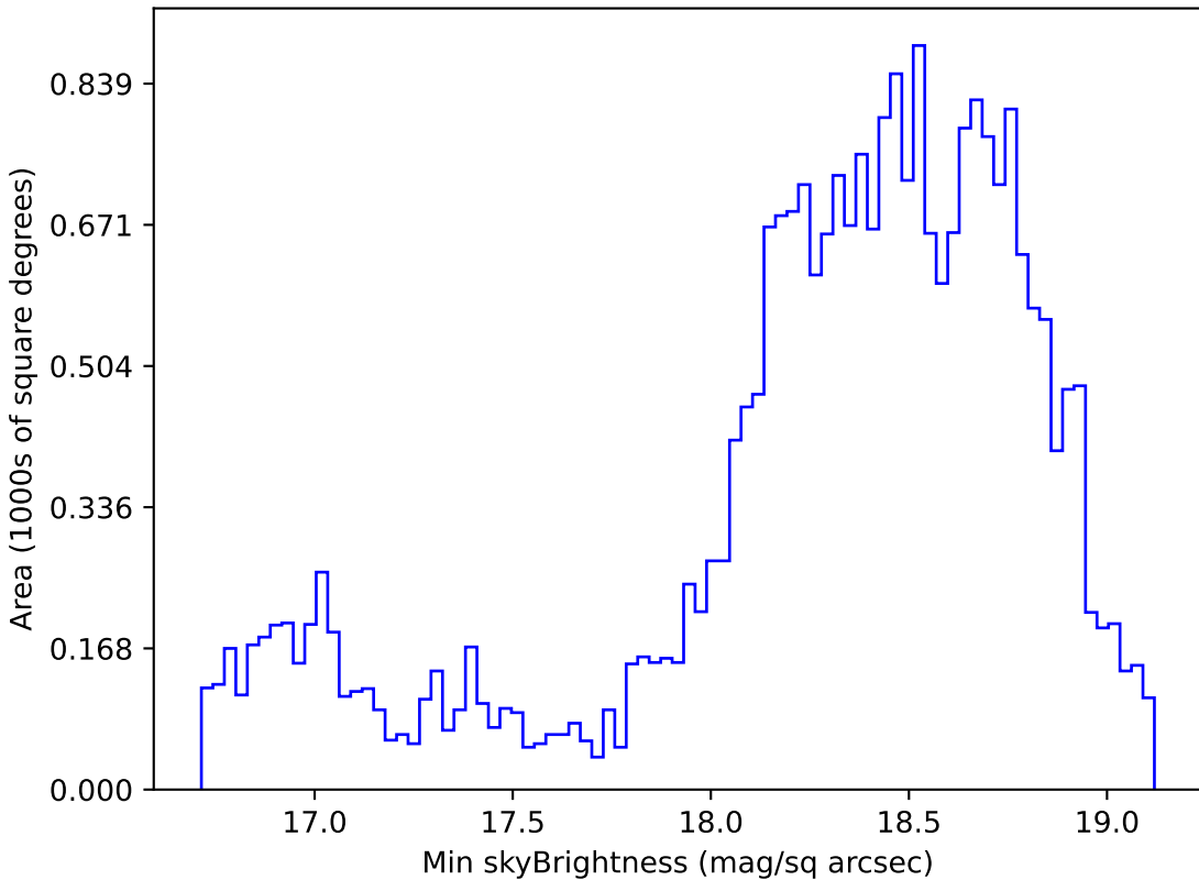
too_ignore_10_1v3.4_10yrs Yr 1 z band: Min skyBrightness
