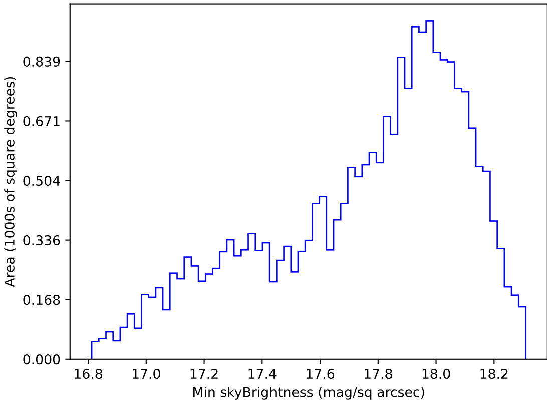
too_ignore_10_1v3.4_10yrs Yr 1 y band: Min skyBrightness
