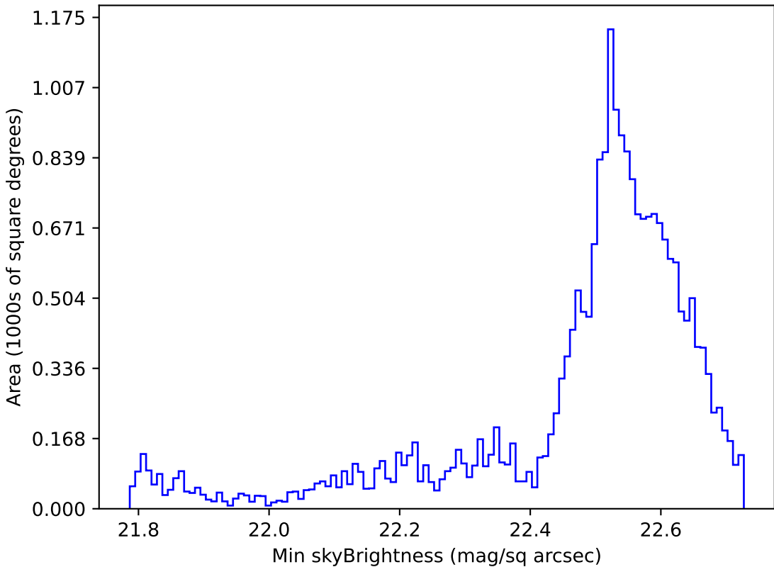
too_ignore_10_1v3.4_10yrs Yr 1 u band: Min skyBrightness
