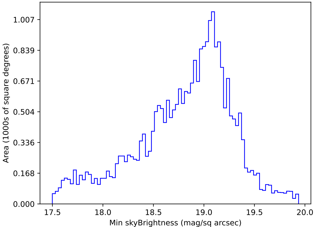
too_ignore_10_1v3.4_10yrs Yr 1 i band: Min skyBrightness
