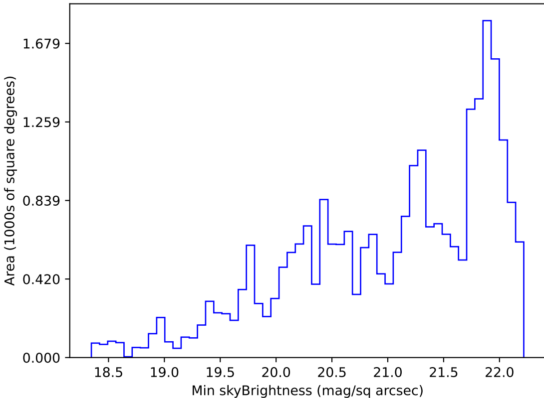
too_ignore_10_1v3.4_10yrs Yr 1 g band: Min skyBrightness
