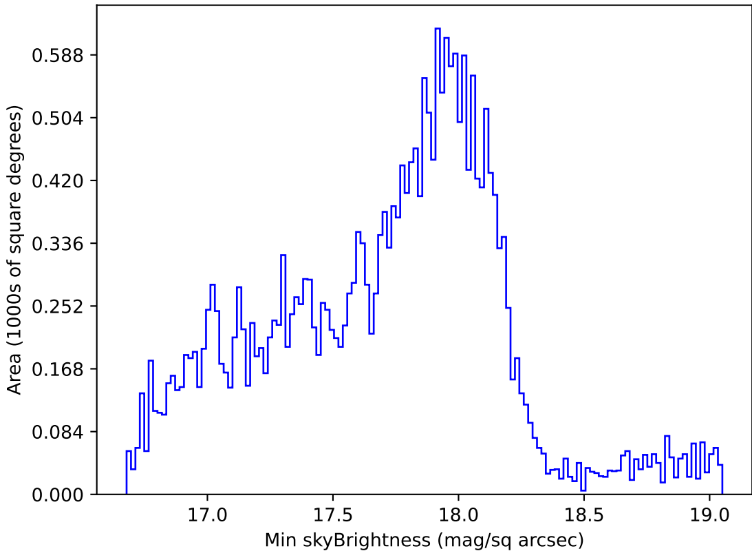
too_ignore_10_1v3.4_10yrs Yr 1 all bands: Min skyBrightness
