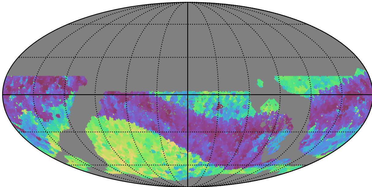
too_ignore_10_1v3.4_10yrs WFD z band: Min skyBrightness
