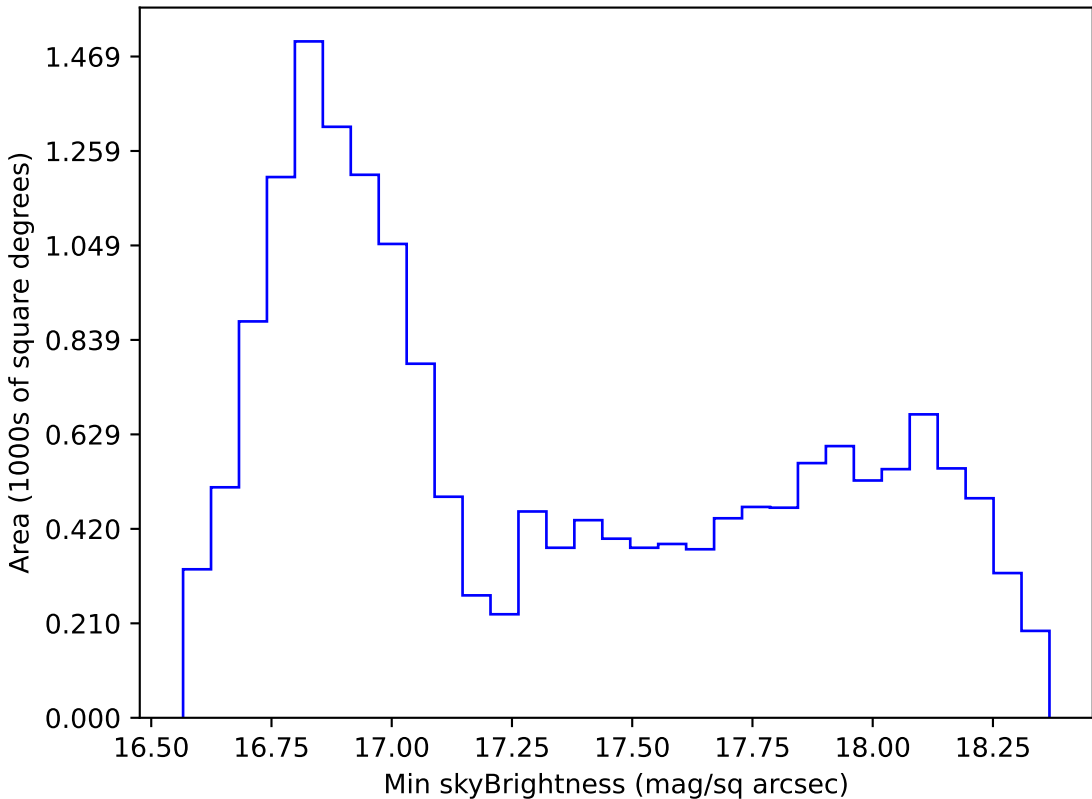
too_ignore_10_1v3.4_10yrs WFD z band: Min skyBrightness
