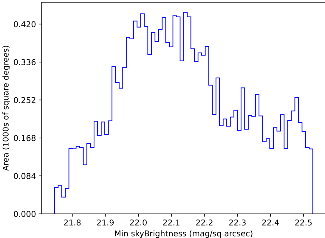
too_ignore_10_1v3.4_10yrs WFD u band: Min skyBrightness
