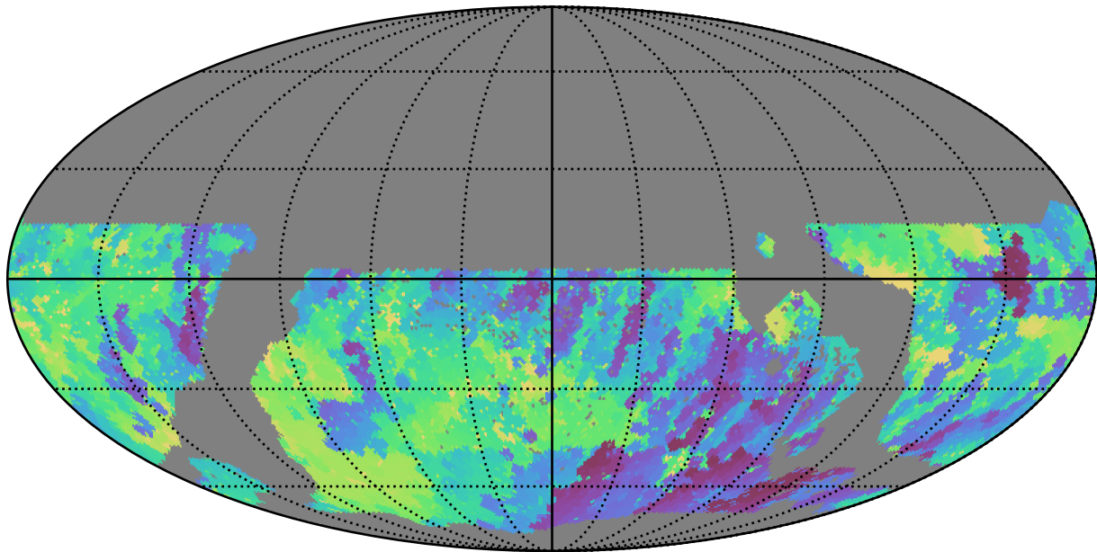
too_ignore_10_1v3.4_10yrs WFD r band: Min skyBrightness
