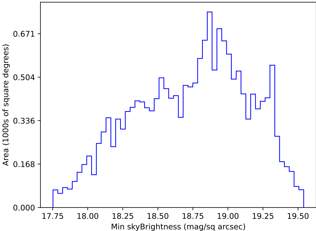
too_ignore_10_1v3.4_10yrs WFD r band: Min skyBrightness
