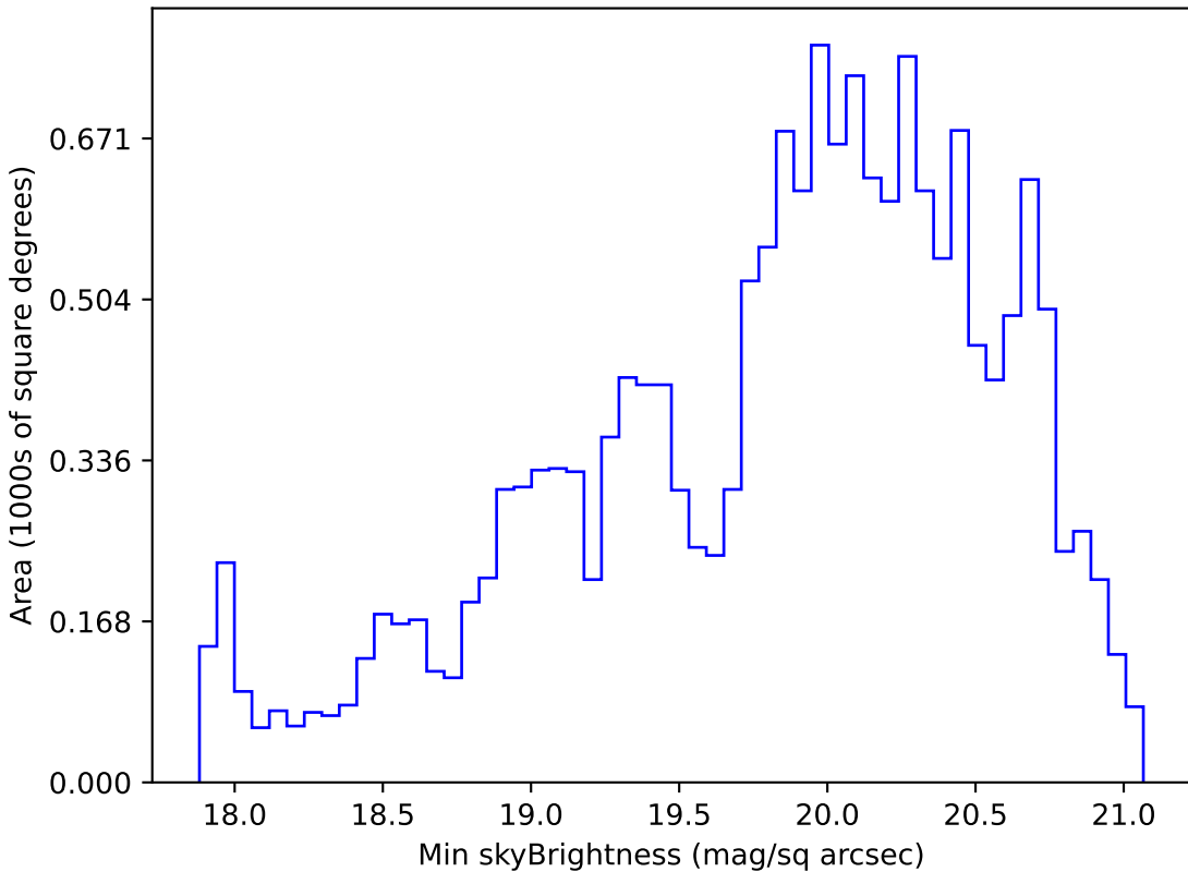
too_ignore_10_1v3.4_10yrs WFD g band: Min skyBrightness
