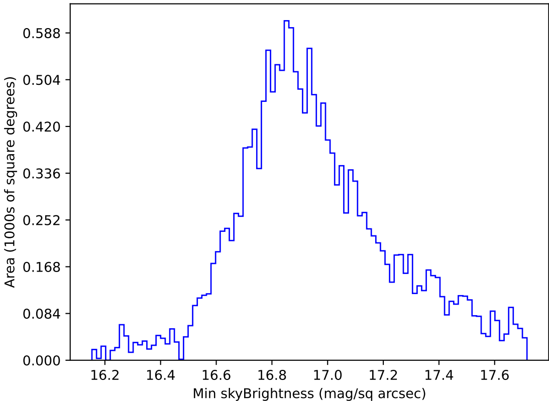
too_ignore_10_1v3.4_10yrs WFD all bands: Min skyBrightness
