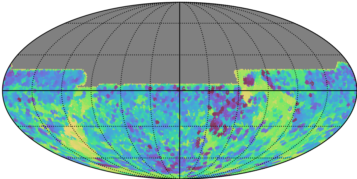
too_ignore_10_1v3.4_10yrs All sky y band: Min skyBrightness
