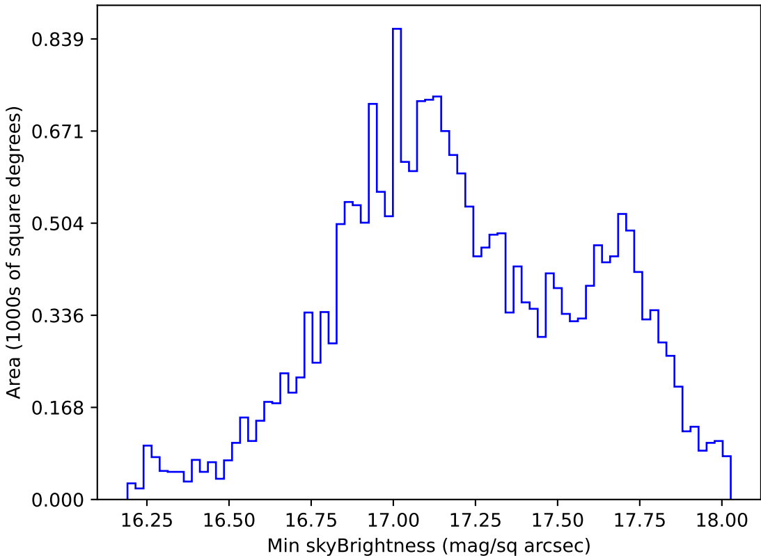
too_ignore_10_1v3.4_10yrs All sky y band: Min skyBrightness
