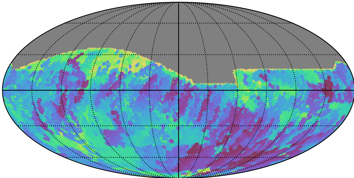
too_ignore_10_1v3.4_10yrs All sky r band: Min skyBrightness
