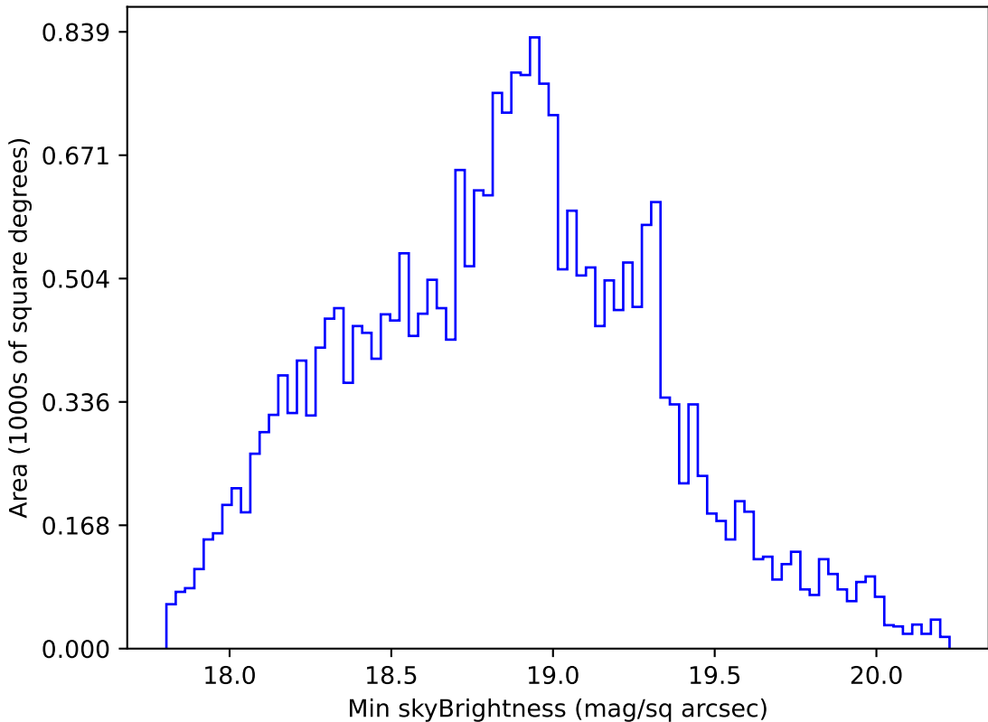
too_ignore_10_1v3.4_10yrs All sky r band: Min skyBrightness
