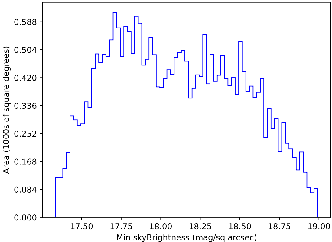
too_ignore_10_1v3.4_10yrs All sky i band: Min skyBrightness
