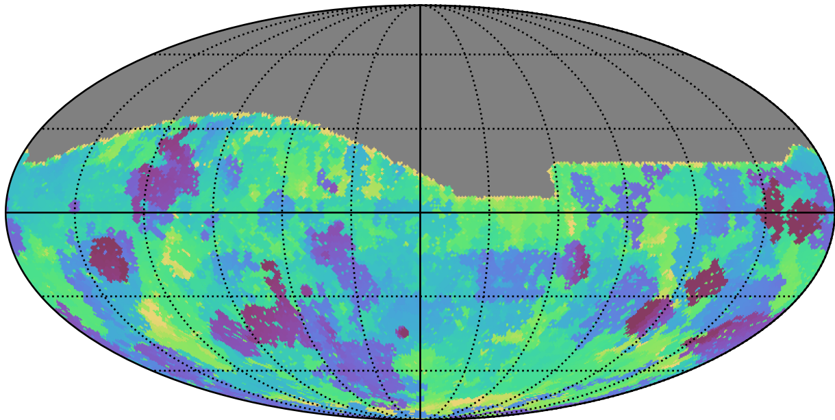
too_ignore_10_1v3.4_10yrs All sky g band: Min skyBrightness
