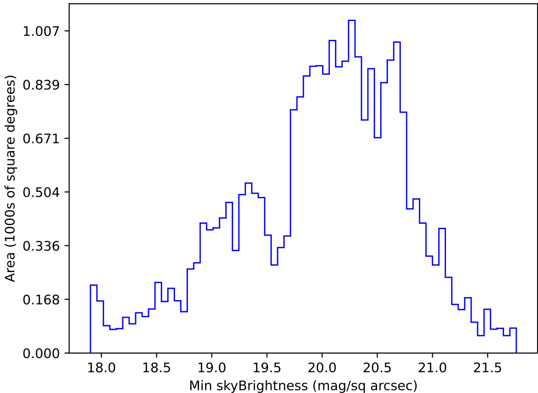
too_ignore_10_1v3.4_10yrs All sky g band: Min skyBrightness
