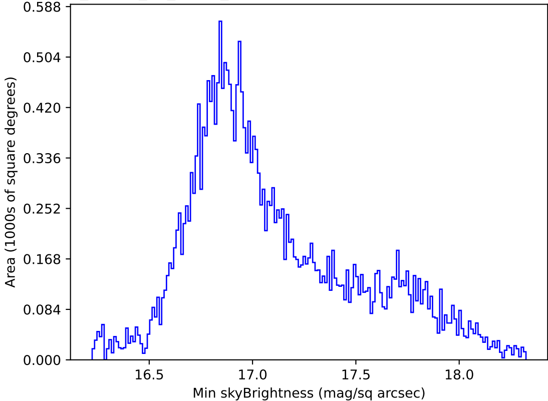
too_ignore_10_1v3.4_10yrs All sky all bands: Min skyBrightness
