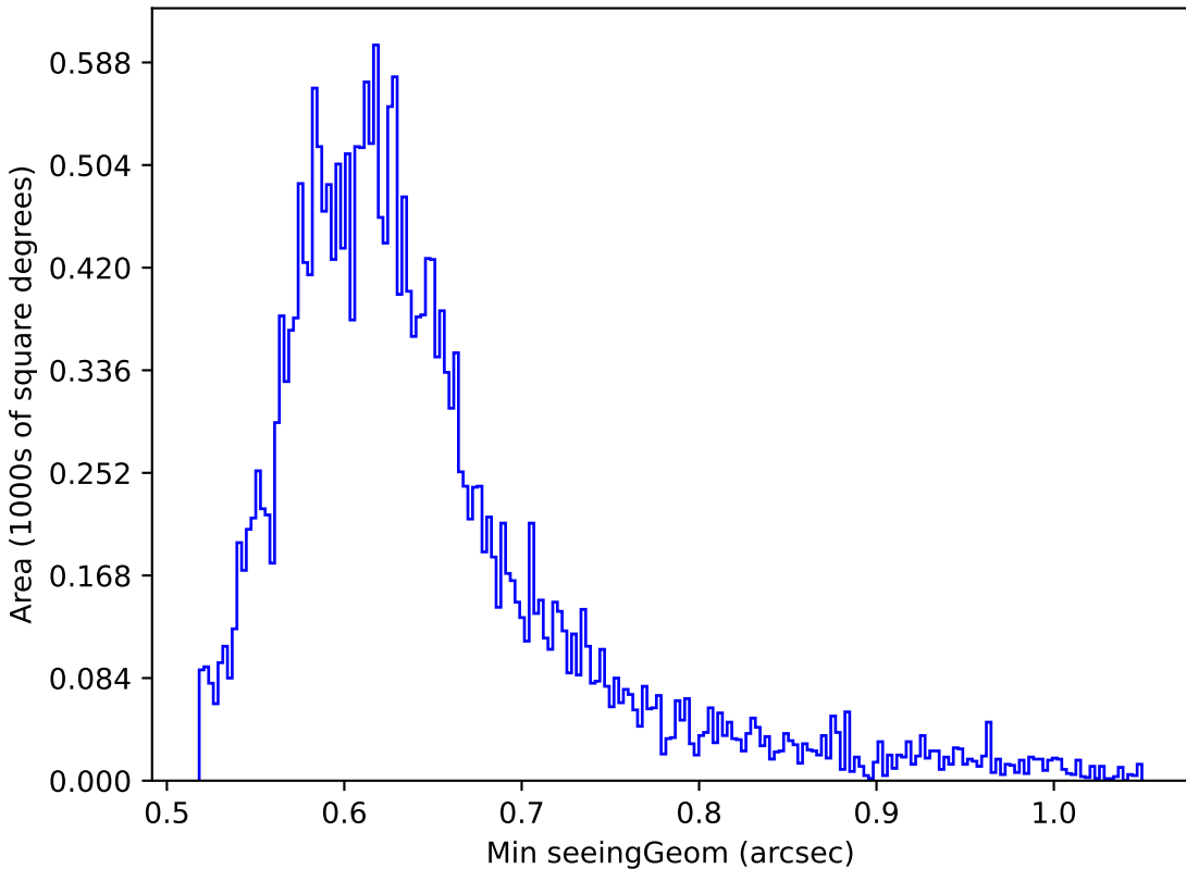
too_ignore_10_1v3.4_10yrs Yr 1 z band: Min seeingGeom
