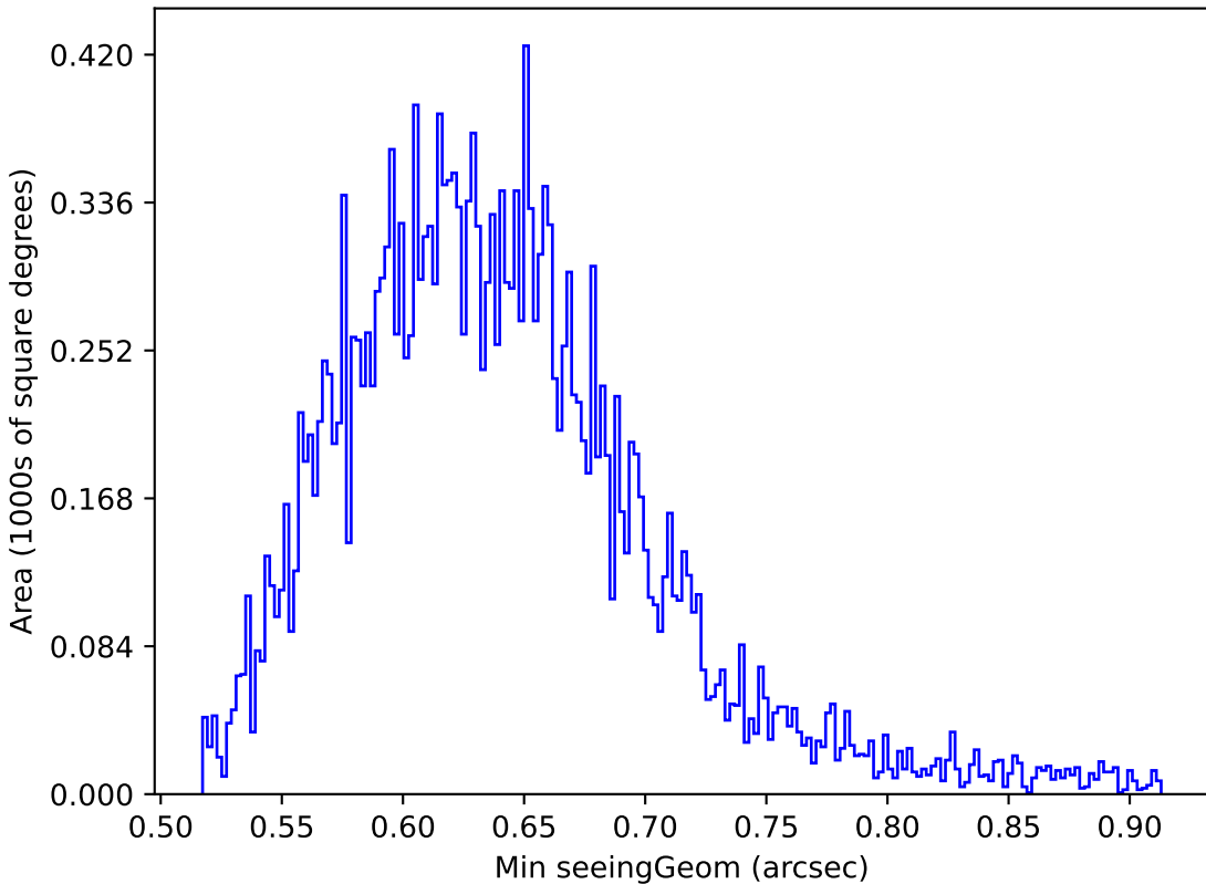
too_ignore_10_1v3.4_10yrs Yr 1 y band: Min seeingGeom
