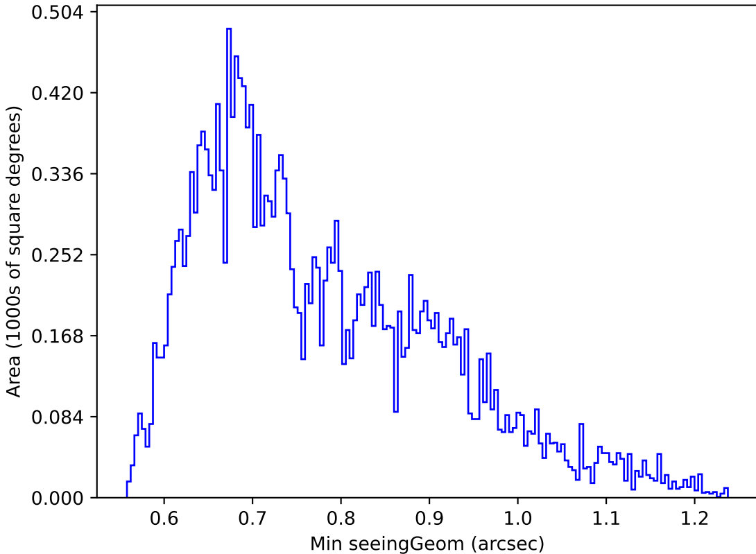
too_ignore_10_1v3.4_10yrs Yr 1 u band: Min seeingGeom
