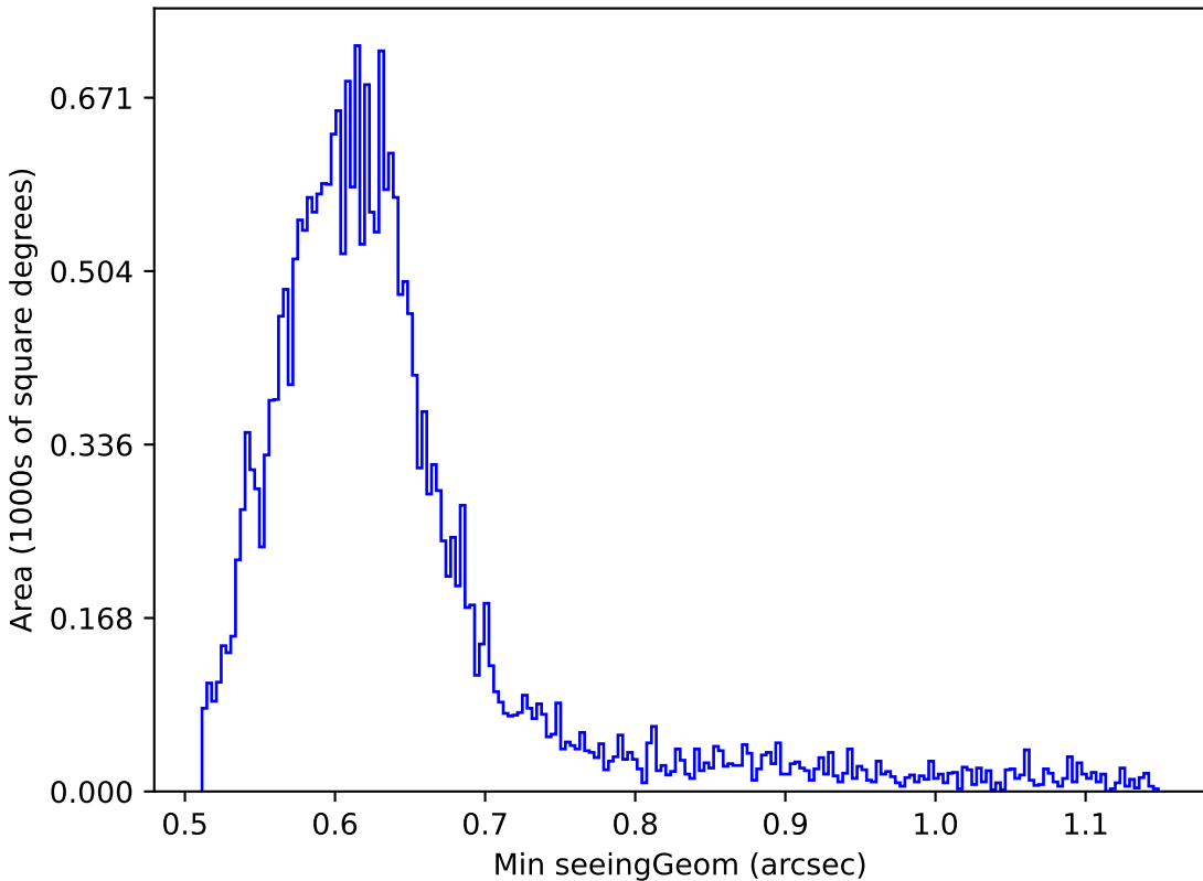
too_ignore_10_1v3.4_10yrs Yr 1 r band: Min seeingGeom
