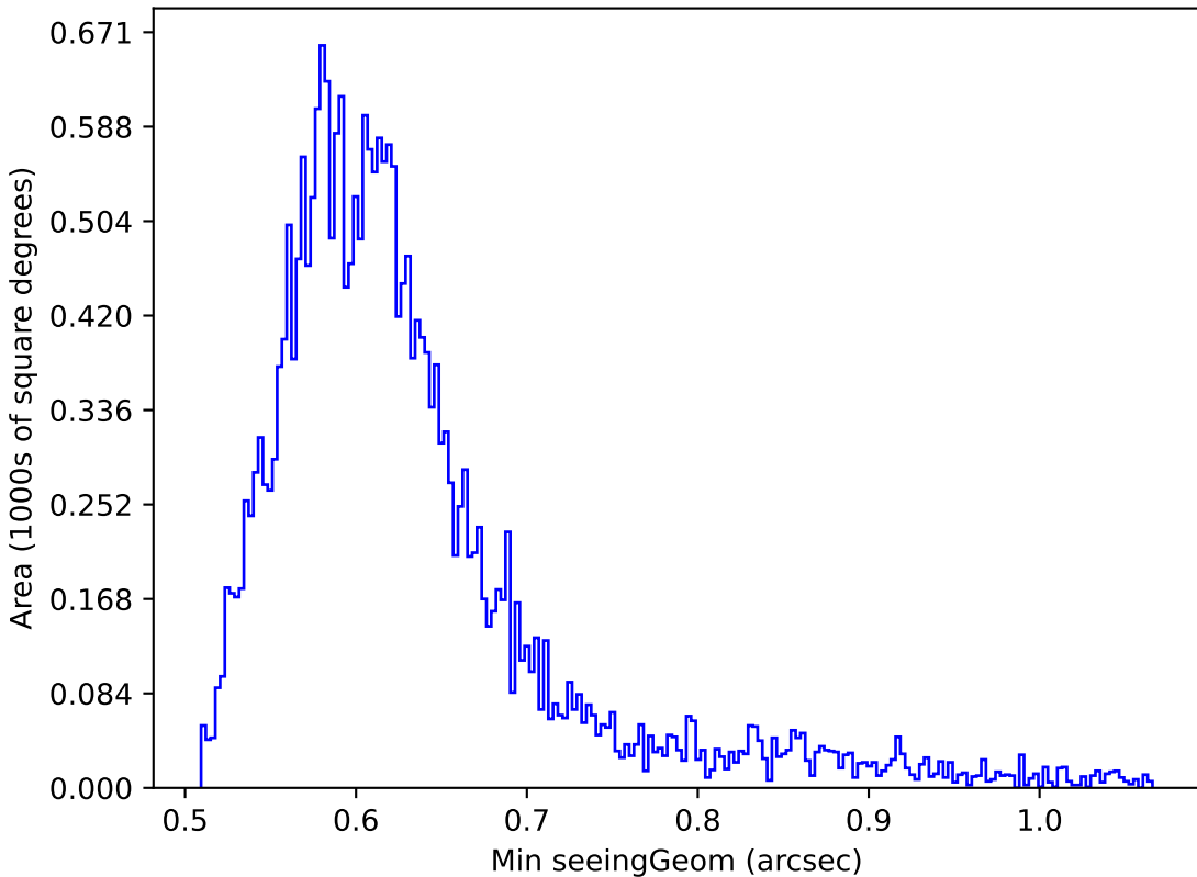
too_ignore_10_1v3.4_10yrs Yr 1 i band: Min seeingGeom
