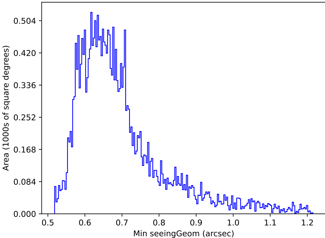
too_ignore_10_1v3.4_10yrs Yr 1 g band: Min seeingGeom
