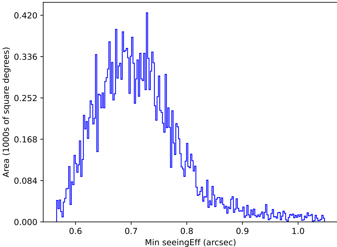
too_ignore_10_1v3.4_10yrs Yr 1 y band: Min seeingEff
