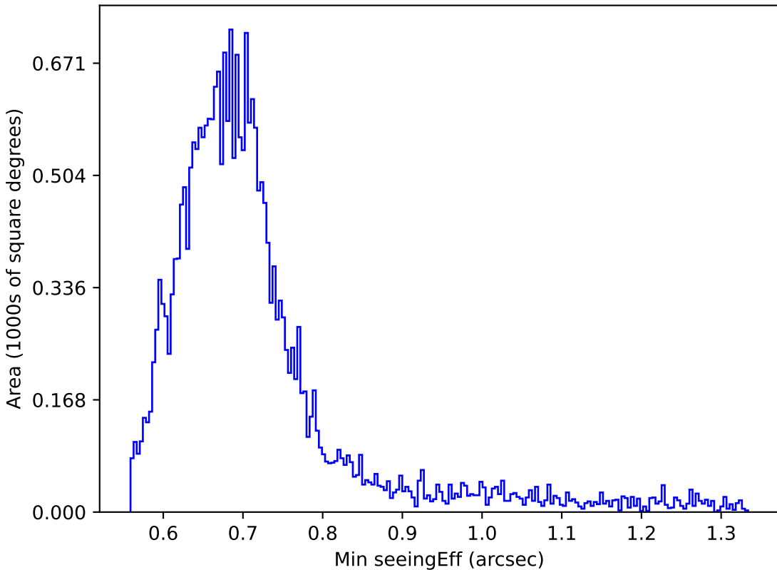
too_ignore_10_1v3.4_10yrs Yr 1 r band: Min seeingEff
