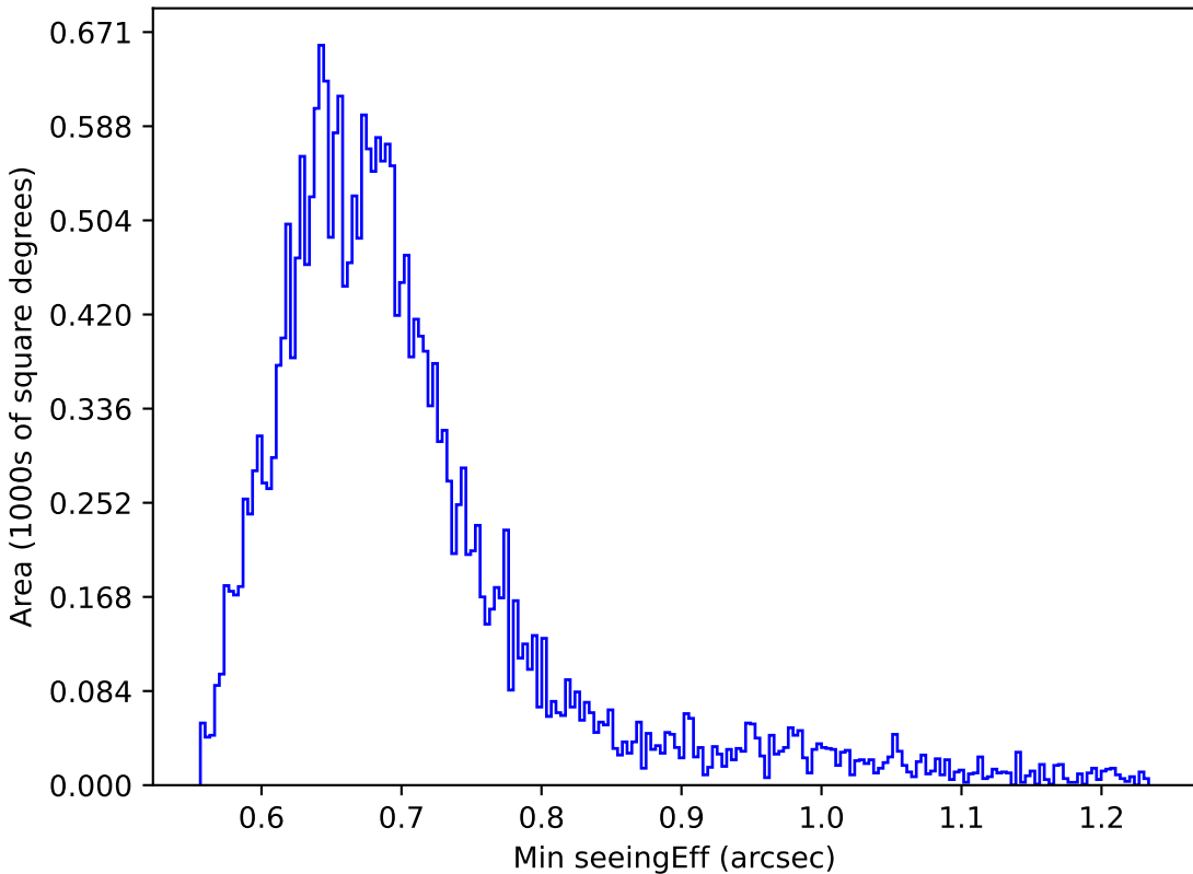
too_ignore_10_1v3.4_10yrs Yr 1 i band: Min seeingEff
