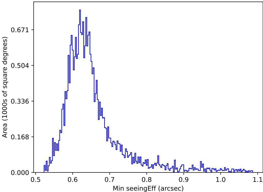
too_ignore_10_1v3.4_10yrs Yr 1 all bands: Min seeingEff
