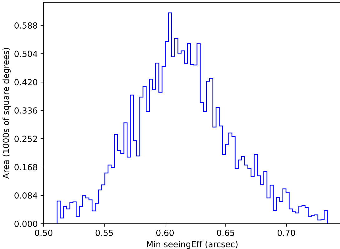
too_ignore_10_1v3.4_10yrs WFD z band: Min seeingEff
