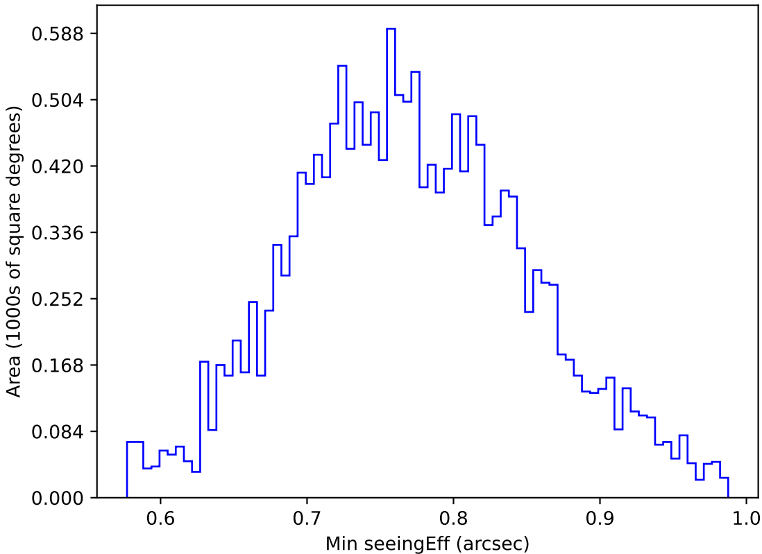
too_ignore_10_1v3.4_10yrs WFD u band: Min seeingEff
