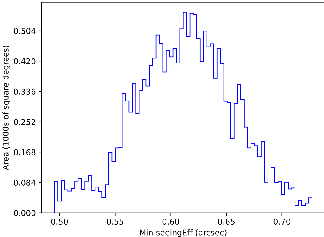
too_ignore_10_1v3.4_10yrs WFD r band: Min seeingEff
