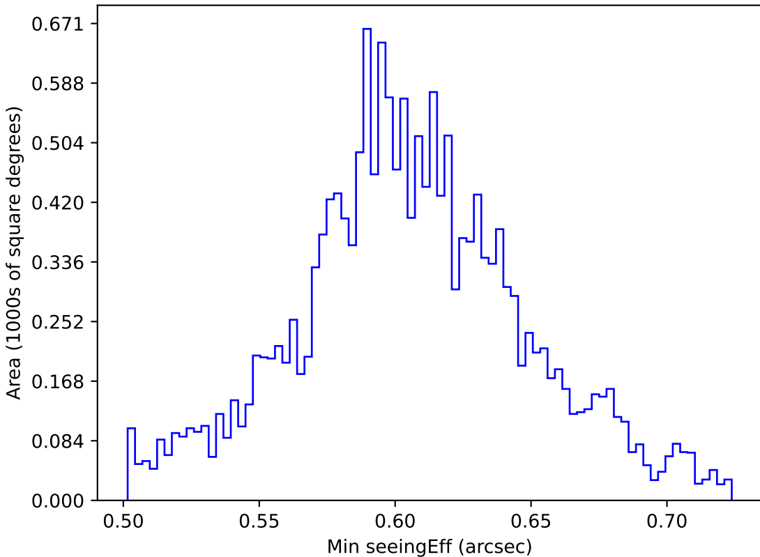
too_ignore_10_1v3.4_10yrs WFD i band: Min seeingEff
