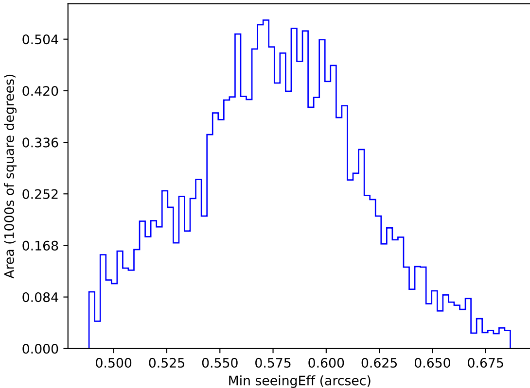
too_ignore_10_1v3.4_10yrs WFD all bands: Min seeingEff
