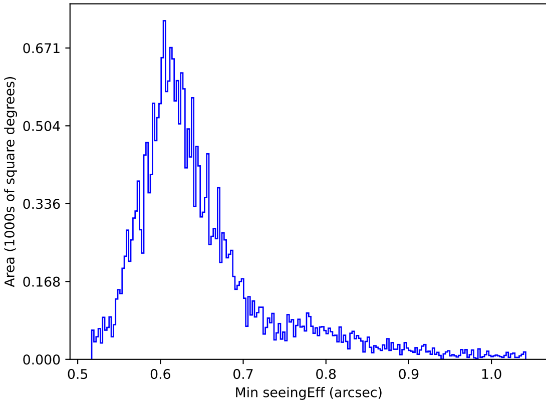
too_ignore_10_1v3.4_10yrs All sky z band: Min seeingEff
