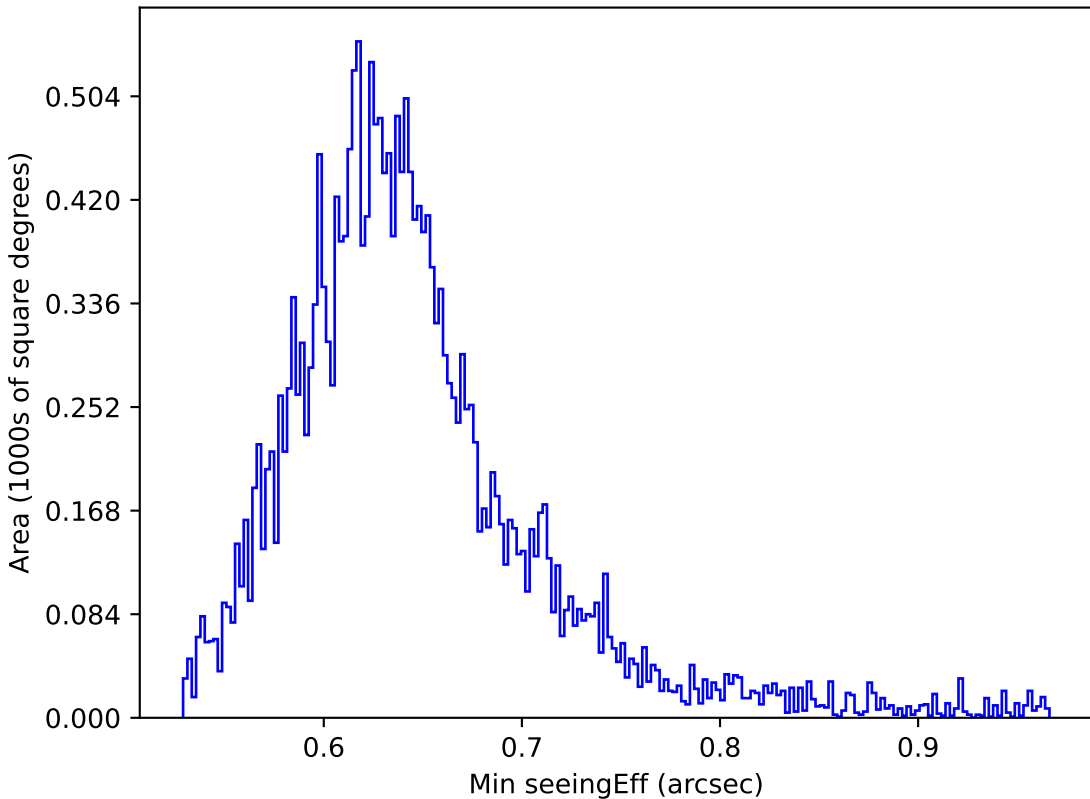
too_ignore_10_1v3.4_10yrs All sky y band: Min seeingEff
