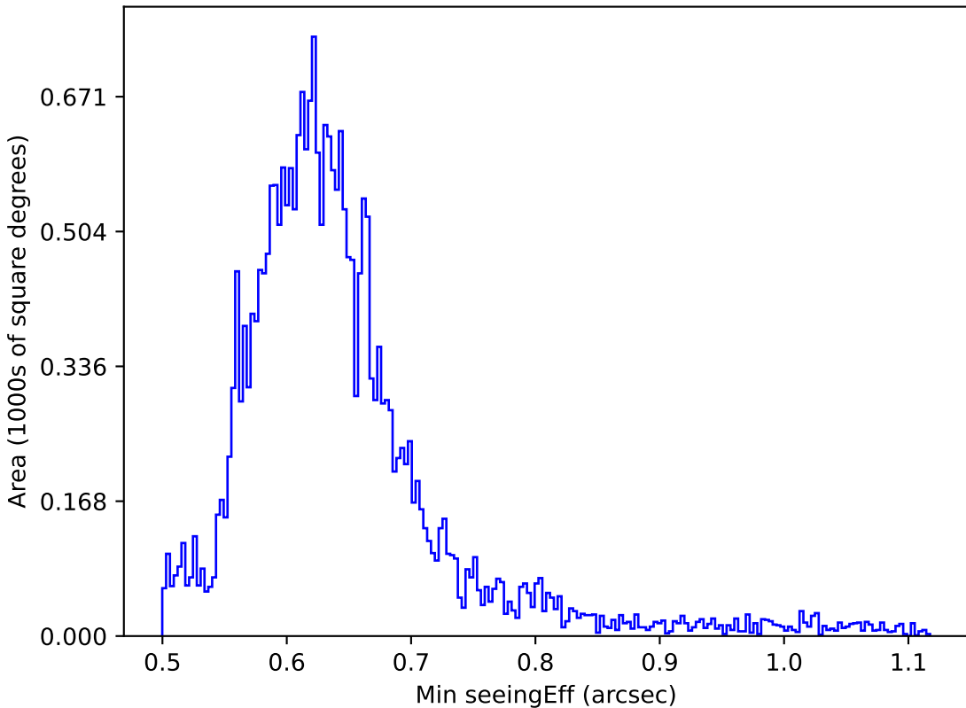
too_ignore_10_1v3.4_10yrs All sky r band: Min seeingEff
