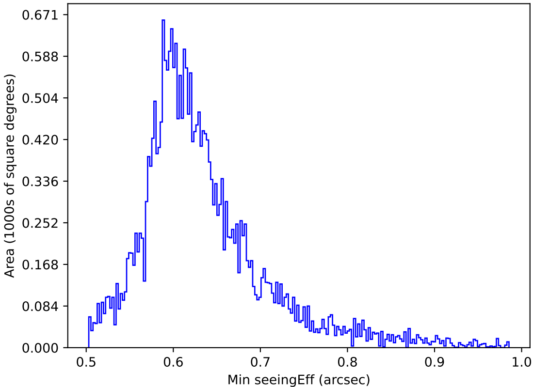
too_ignore_10_1v3.4_10yrs All sky i band: Min seeingEff
