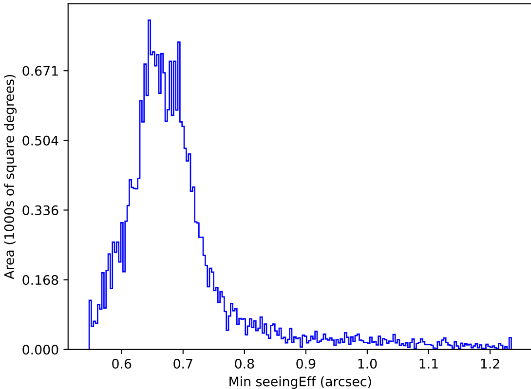
too_ignore_10_1v3.4_10yrs All sky g band: Min seeingEff
