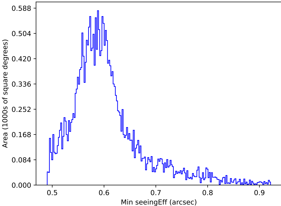
too_ignore_10_1v3.4_10yrs All sky all bands: Min seeingEff
