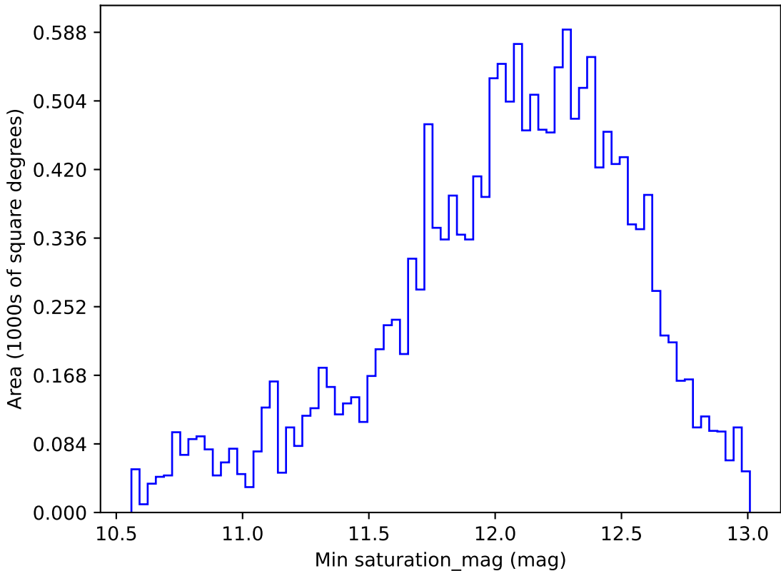
too_ignore_10_1v3.4_10yrs WFD z band: Min saturation_mag
