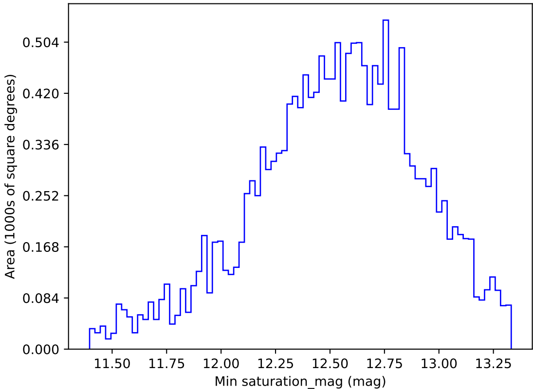
too_ignore_10_1v3.4_10yrs WFD r band: Min saturation_mag
