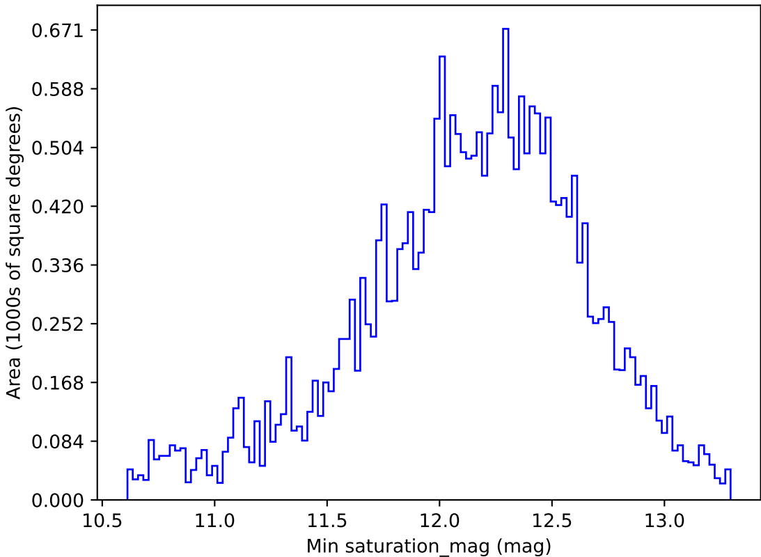
too_ignore_10_1v3.4_10yrs All sky z band: Min saturation_mag
