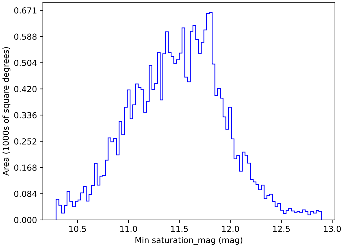
too_ignore_10_1v3.4_10yrs All sky u band: Min saturation_mag
